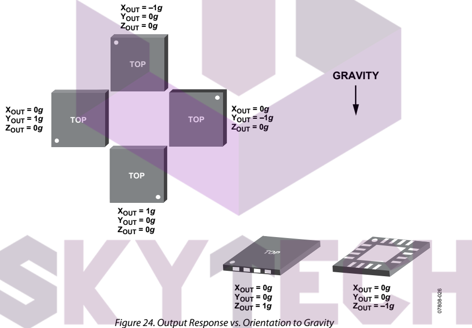
Figure 24. Output Response vs. Orientation to Gravity
